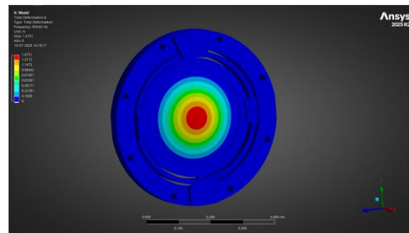
Mode 8 — 959.83 Hz
