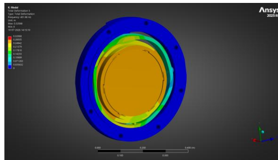
Mode 3 — 401.96 Hz
