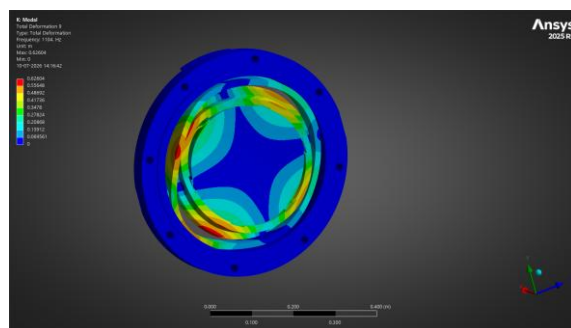
Mode 9 — 1104.0 Hz
