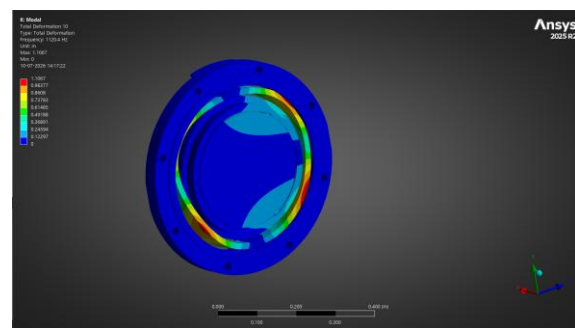
Mode 10 — 1120.4 Hz
