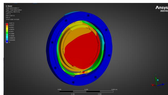
Mode 2 — 400.73 Hz
