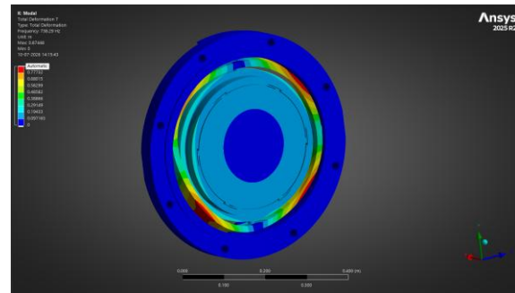
Mode 7 — 738.29 Hz
